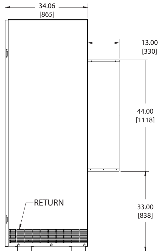
RIGHT VIEW
