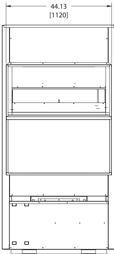
REAR VIEW
