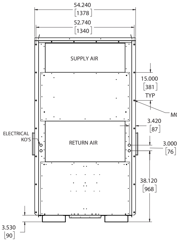
REAR VIEW
