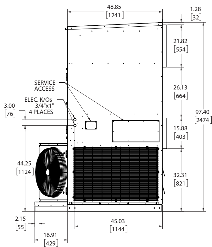
RIGHT VIEW
