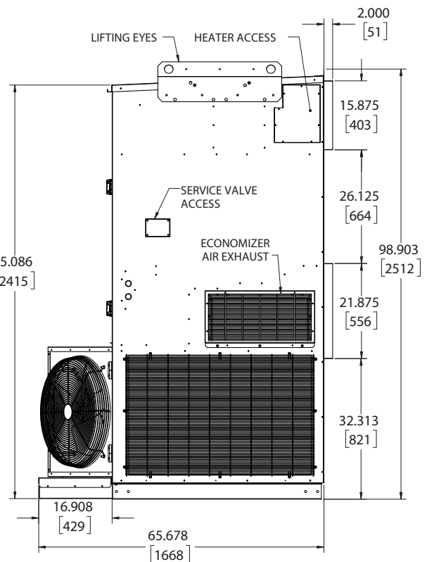
RIGHT VIEW
