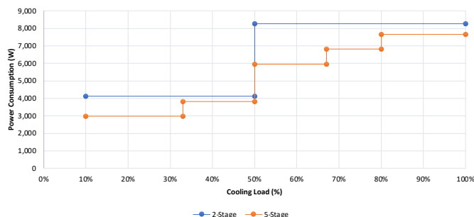
Figure 2: Power Consumption Vs. Cooling Demand
