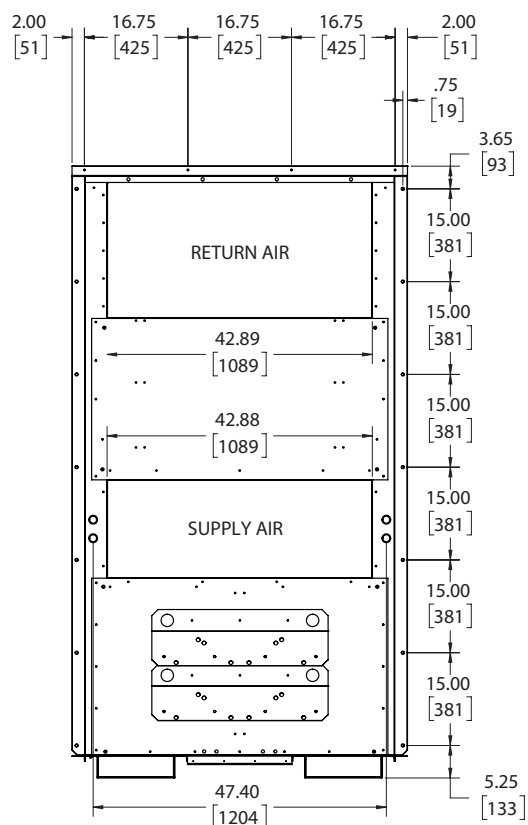
REAR VIEW
